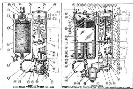
PLATE 16 - VACUUM CONTROL, FUEL FILTER AND TRANSFER PUMP
