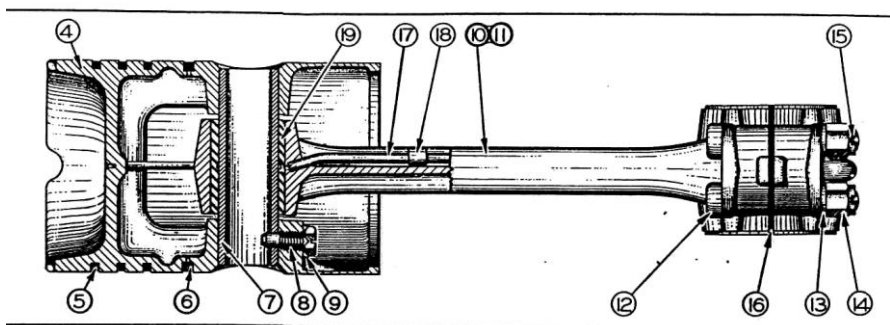
PLATE 3 - PISTON AND CONNECTING ROD
