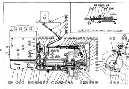
PLATE 14 - GOVERNOR AND INJECTION PUMP DRIVE
