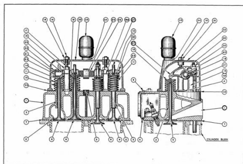
PLATE 12 - CYLINDER HEAD
