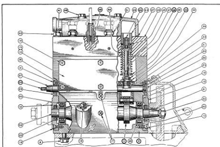
PLATE 15 - INJECTION PUMP
